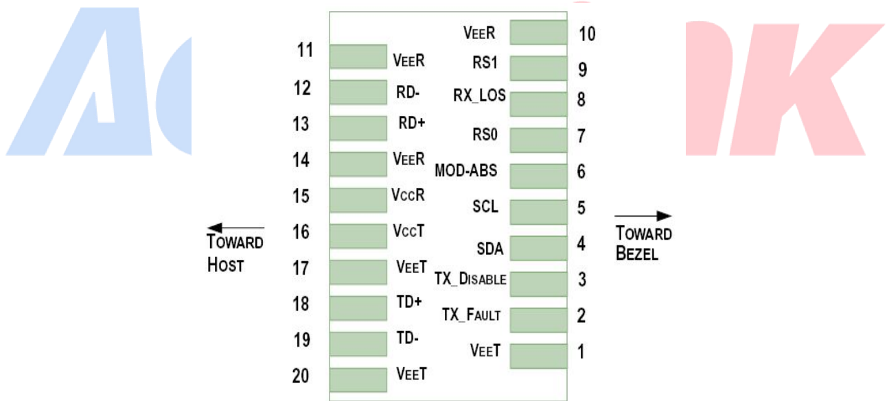
Figure 2. Pin function definitions
