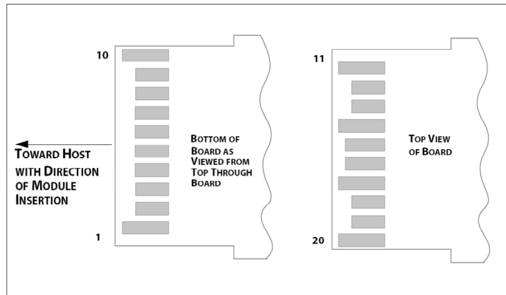
SFP+ Transceiver Electric Pad Layout
