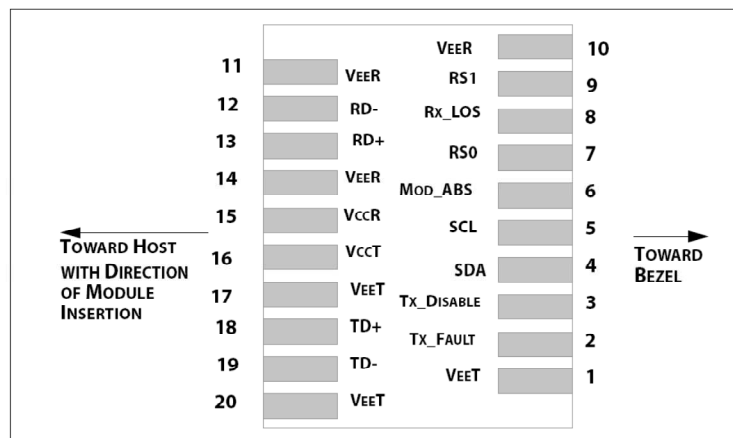
SFP+ Transceiver Host PCB PAD Assignment
